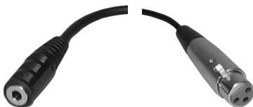
44-182 (WIRING A) 44-184 (WIRING B)
