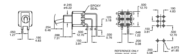
DPDT
