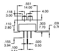
P.C. MOUNTING
