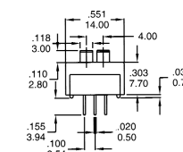
P.C. MOUNTING
