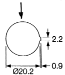
PANEL CUT-OUT (mm)
