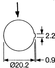
PANEL CUT-OUT (mm)
