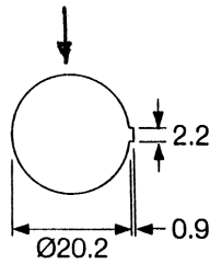
PANEL CUT-OUT (mm)
